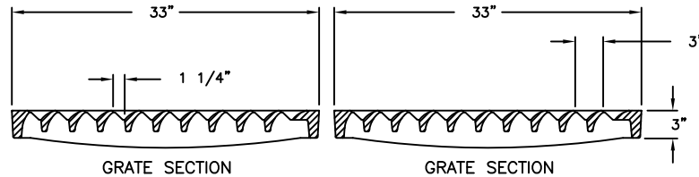
GRATE SECTION
