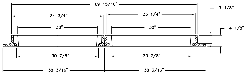
FRAME SECTION
