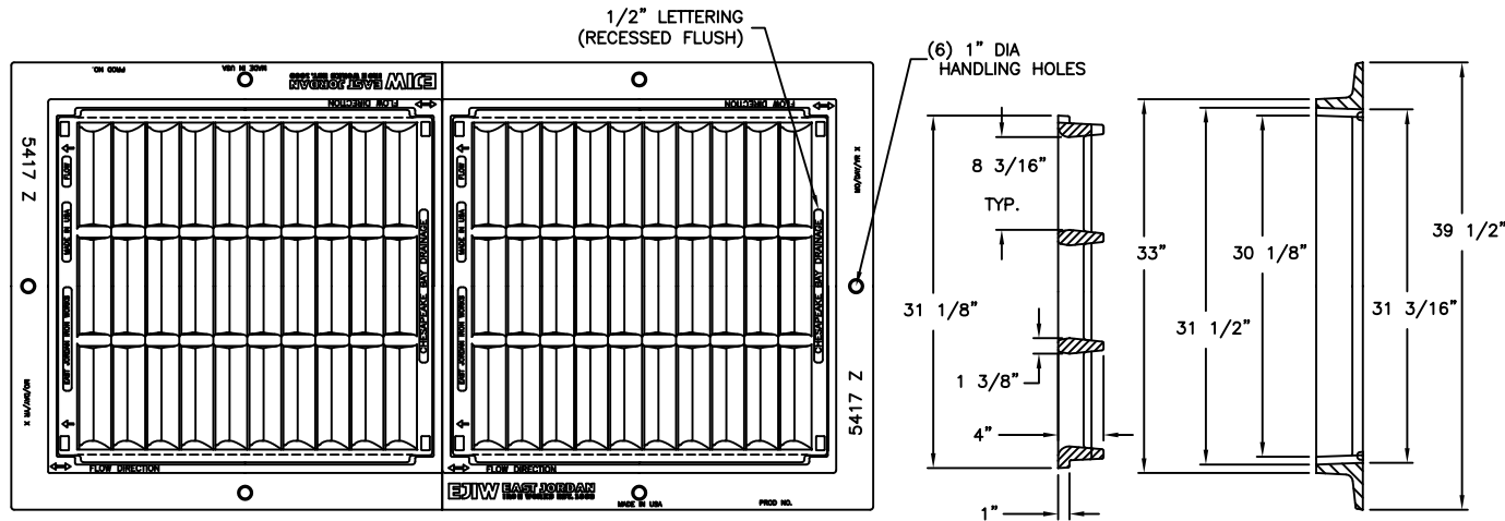
FRAME SECTION
